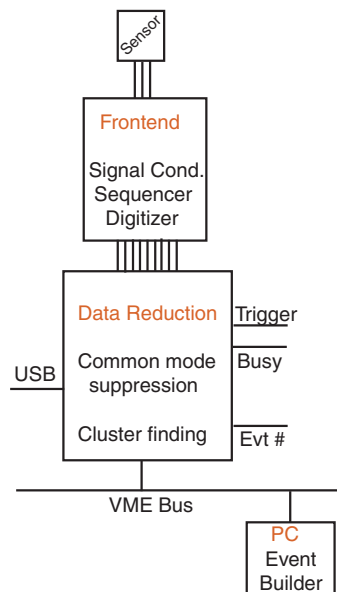
Fig. 3. Schematic layout of the DAQ system.
