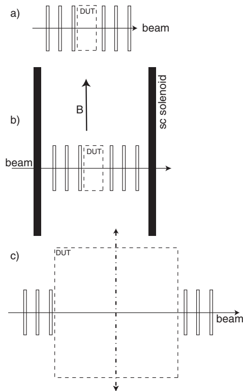
Fig. 2. Three foreseen layouts for the beam telescope; (a) a compact layout for characterization of high precision devices, (b) a compact layout inside a magnetic field and (c) a two-arm geometry for the use with larger DUTs.
