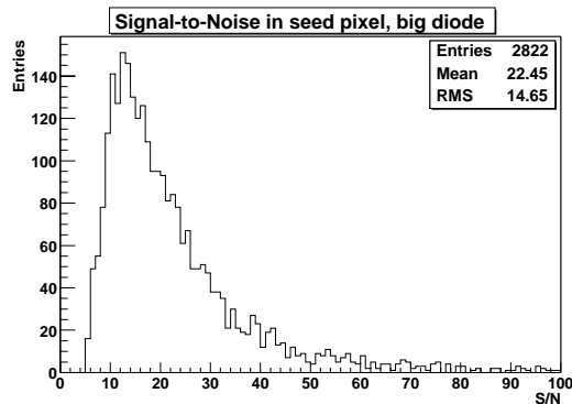
Fig. 1. Signal-to-noise distribution for 6 GeV/c electrons for an individual seed pixel in a MIMOSA-5 CMOS sensor operated at -10^\circ \text{ C} .
