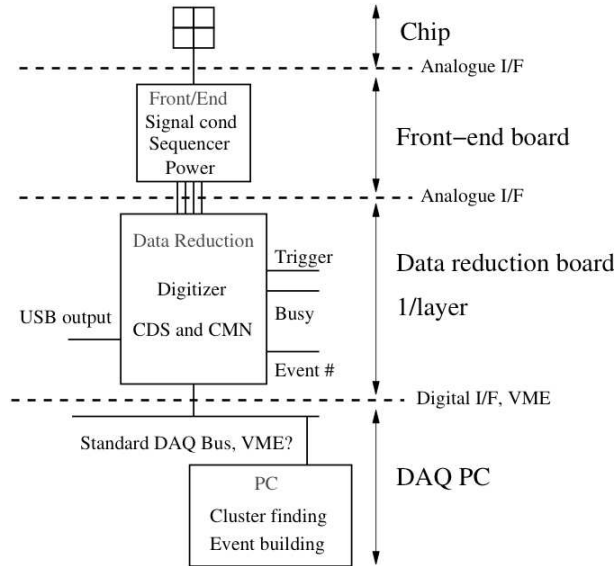
Figure 1: Design of the DAQ system for the high resolution pixel telescope.
