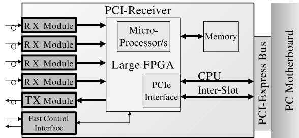
Figure 2: Off-detector receiver design for calorimeters.
